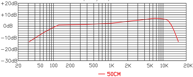
Frequency Respond
